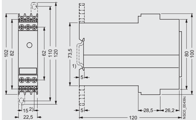
3RG78 57-1BD evaluation unit
