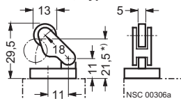
Roller lever, Type E
