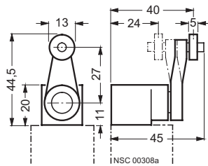
Twist lever, adjustable length
