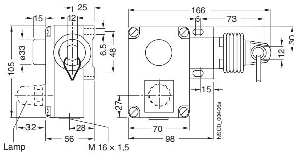
3SE7 160-1AE.. with latching and button reset
