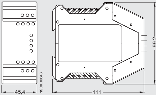
3RG78 25 evaluation unit
