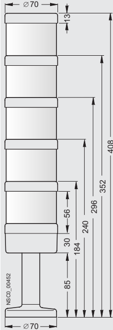
Signaling column (5-tier)
