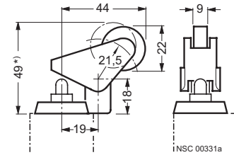
Angular roller lever
